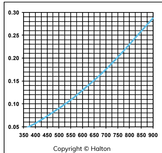
KVM - 2.5 Filters
