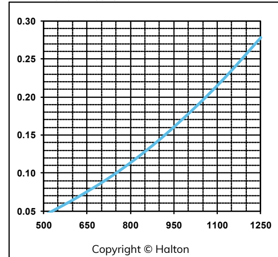
KVM - 3.5 Filters
