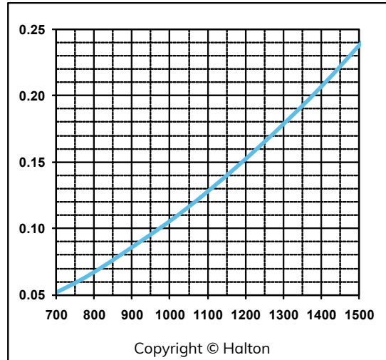
KVM - 4.5 Filters
