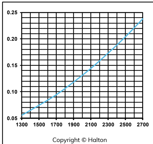
KVM - 9 Filters
