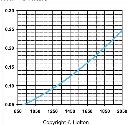
KVM - 6 Filters
