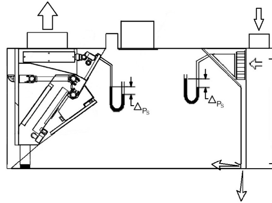
Exhaust air flow vs. pressure differential
