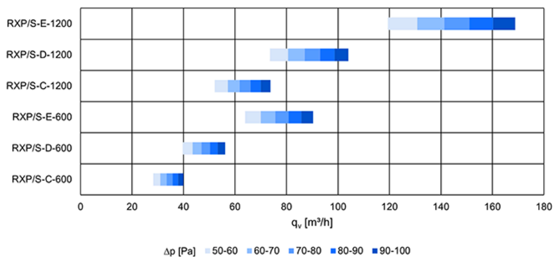
Fig. 13. Airflow ranges in m³/h for Halton Rex RXP, Standard model without HAQ/with HAQ closed with different static chamber pressure levels
